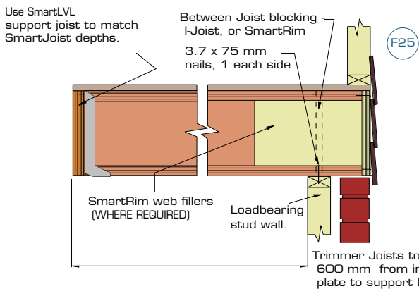
TRIMMER JOISTS WHERE MAIN JOISTS RUN PARALLEL TO BRICK LEDGE CANTILEVER WALL.
