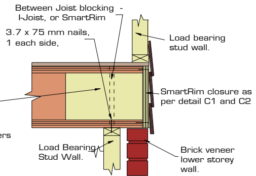
REINFORCING GUIDELINES (a) USING WEB FILLERS
